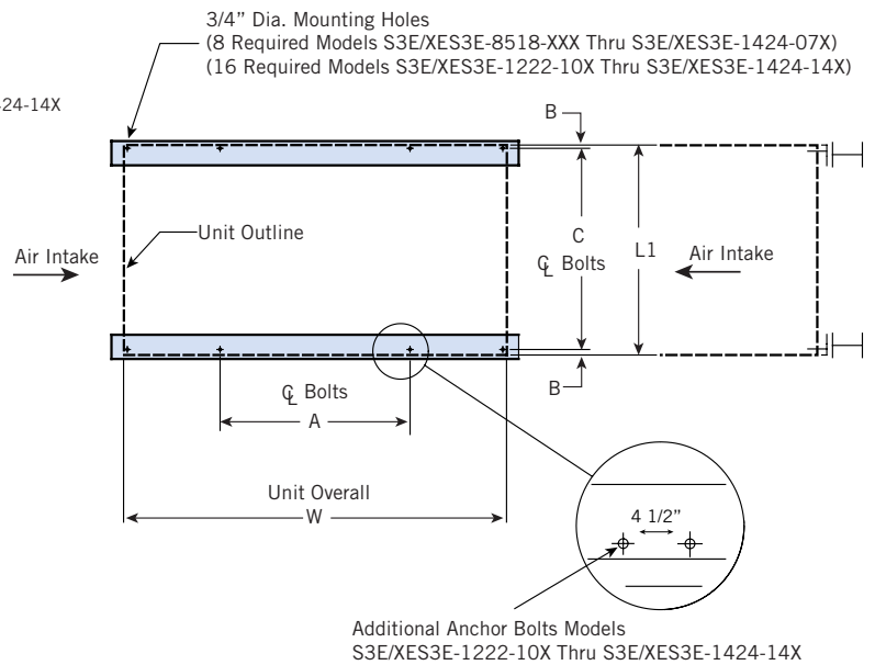
Plan B: Single Cell Unit
