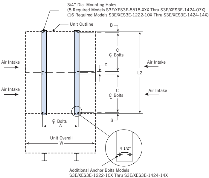
Plan C: Double Cell Unit
