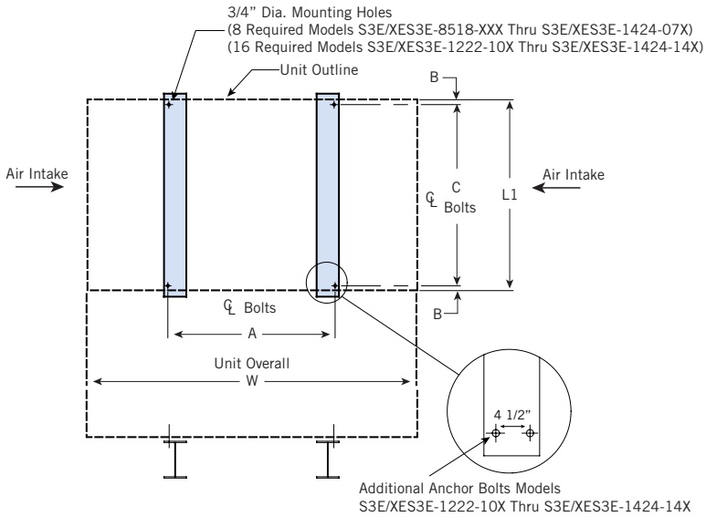
Plan A: Single Cell Unit
